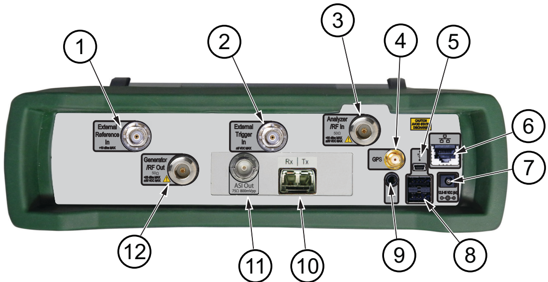
Figure 2-14. Spectrum Master Connector Panel
